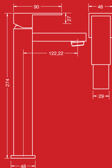
Tall Basin Mixer ( WELS 4 Star, 7 L/min ) ALS-SCTB
