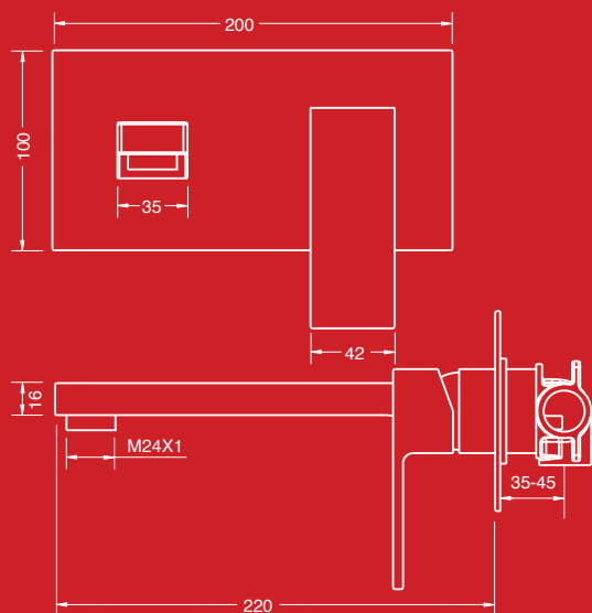
Wall Mixer/Spout ( WELS 4 Star, 7 L/min ) ALS-SCW&S
