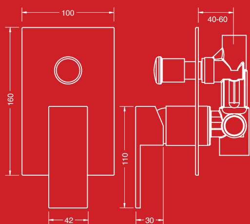
Wall Mixer with Divertor ALS-SCD
