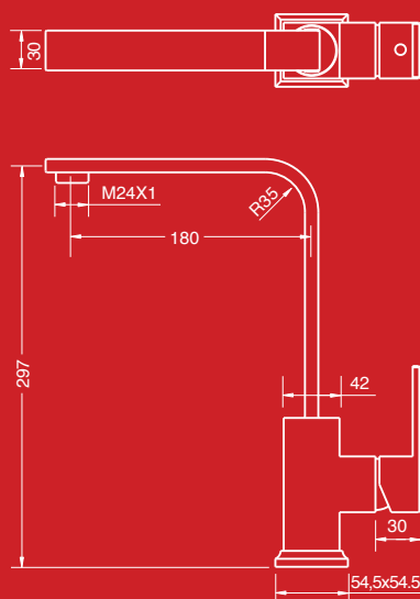
Sink Mixer ( WELS 4 Star, 7 L/min ) ALS-SCS
