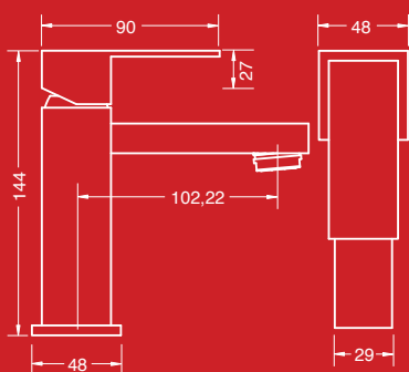
Basin Mixer ( WELS 4 Star, 7 L/min ) ALS-SCB1
