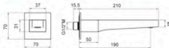
Bath Spout Style TW320 polished chrome
