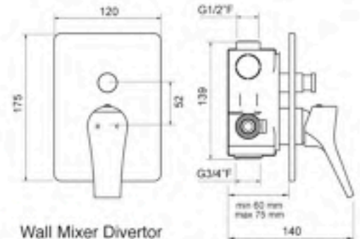
Wall Mixer Divertor Style TW310 polished chrome
