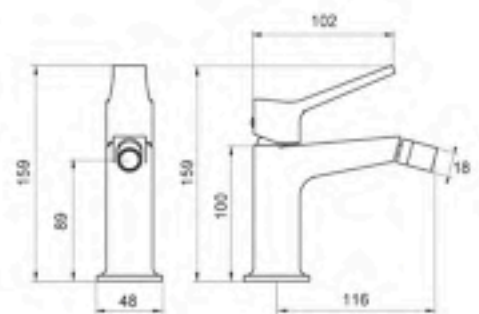
Bidet Mixer Style TW220 polished chrome
