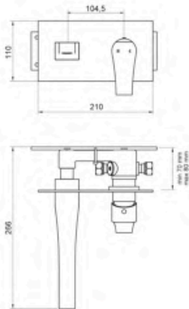
Wall Mixer/Spout Style TW206 polished chrome
