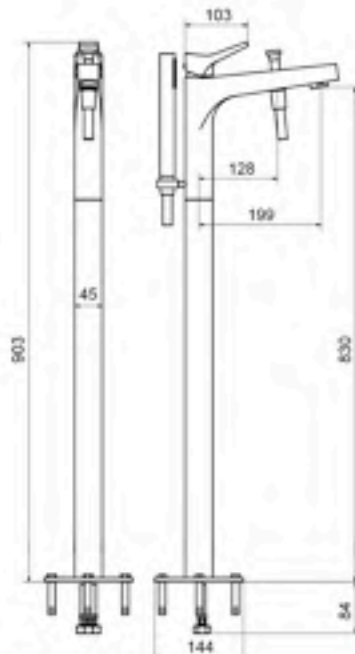
Bath Filler Style TW399 polished chrome
