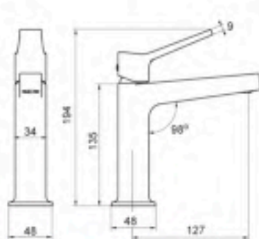
Basin Mixer Style TW200 polished chrome
