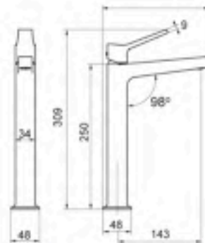
Tall Basin Mixer Style TW202 polished chrome
